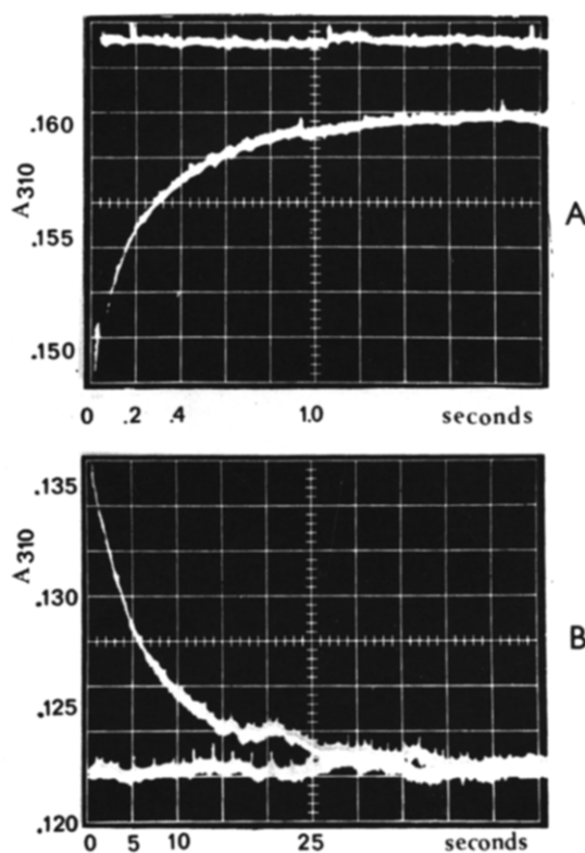
Fig. 2. Kinetics of \text{Mg}^{2+} -induced ribosomal subunit association (2 A) and EDTA-induced 70 S ribosome dissociation (2 B): A) mixing of ribosome solution in 1 mM \text{Mg}^{2+} with a 30 mM \text{Mg}^{2+} buffered solution. Time scale on abscissa: 0.2 sec/division; B) mixing of ribosome solution in 30 mM \text{Mg}^{2+} with a 100 mM EDTA buffered solution. Time scale on abscissa: 5 sec/division. Absorbance at 310 nm on ordinate (A and B), 0.002/division.
